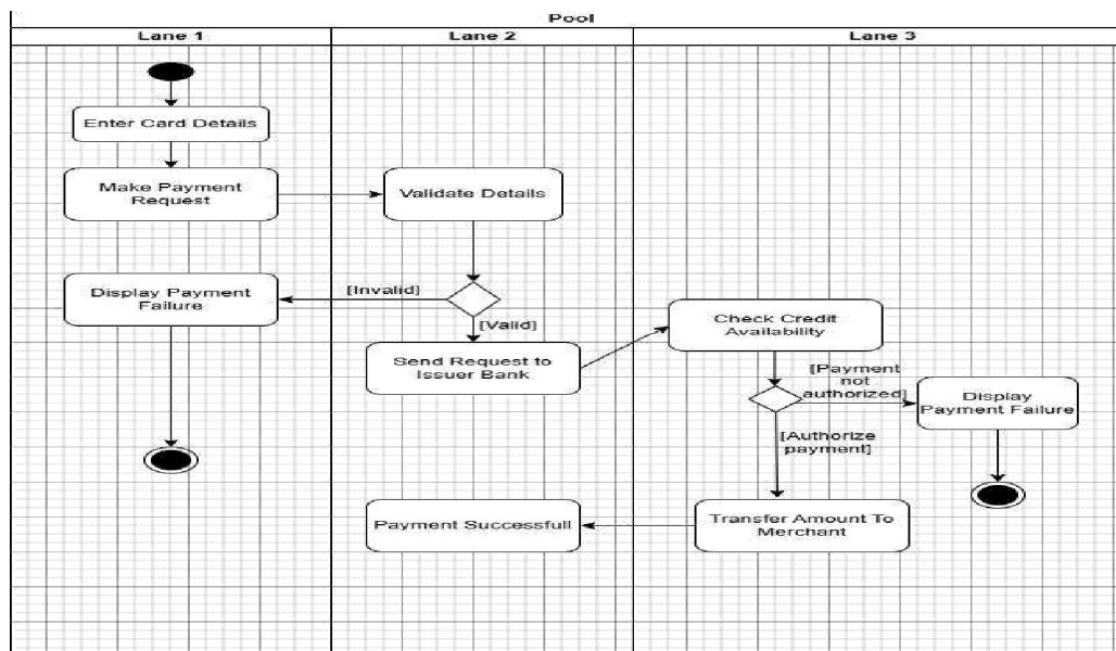
Fig 2.9 Advanced Activity diagram CCMS
