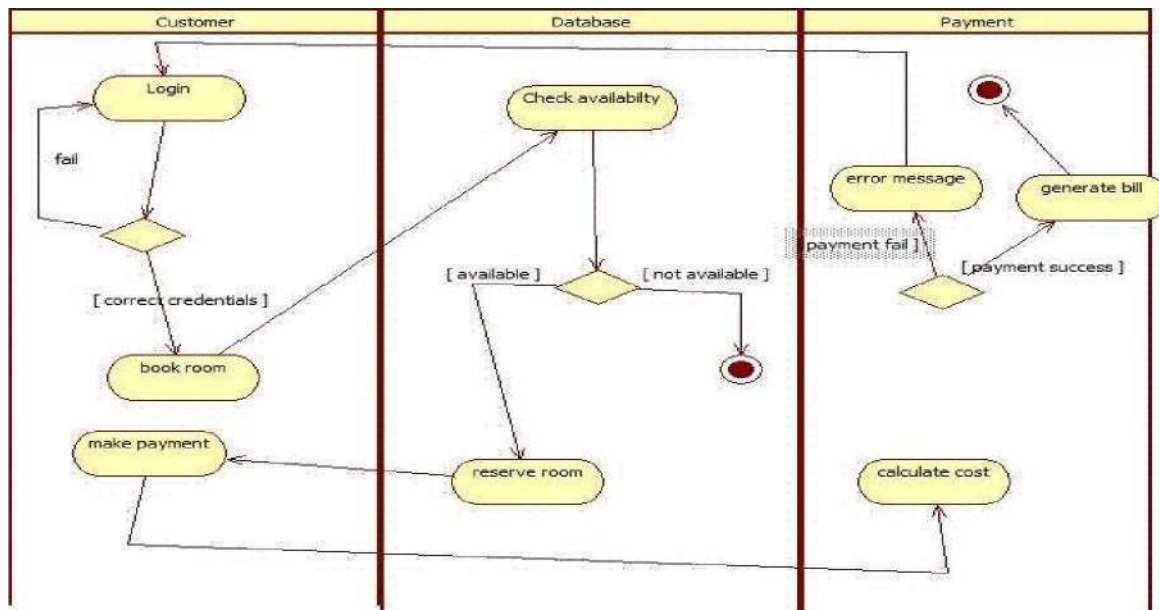
Fig 1.8 Simple activity diagram HMS
