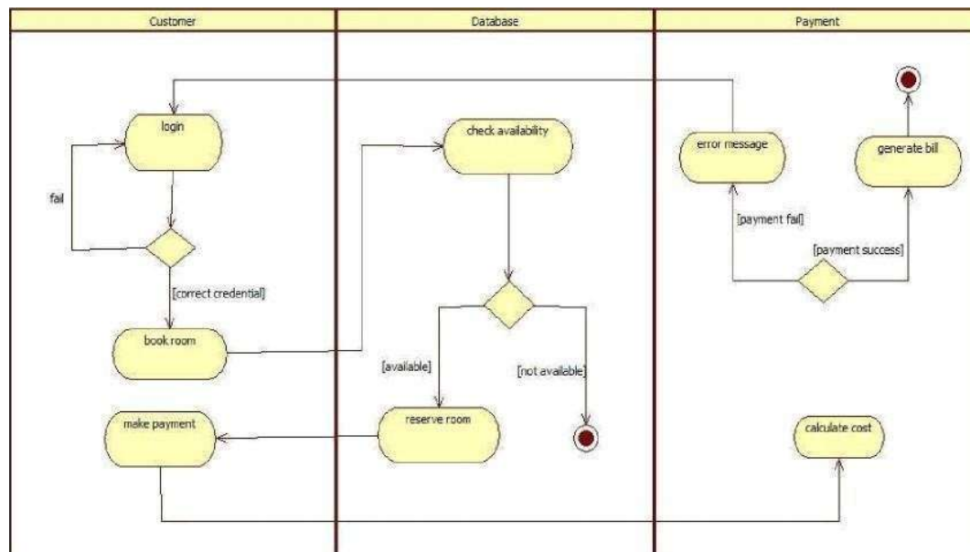
Fig 1.9 Advanced activity diagram for HMS
