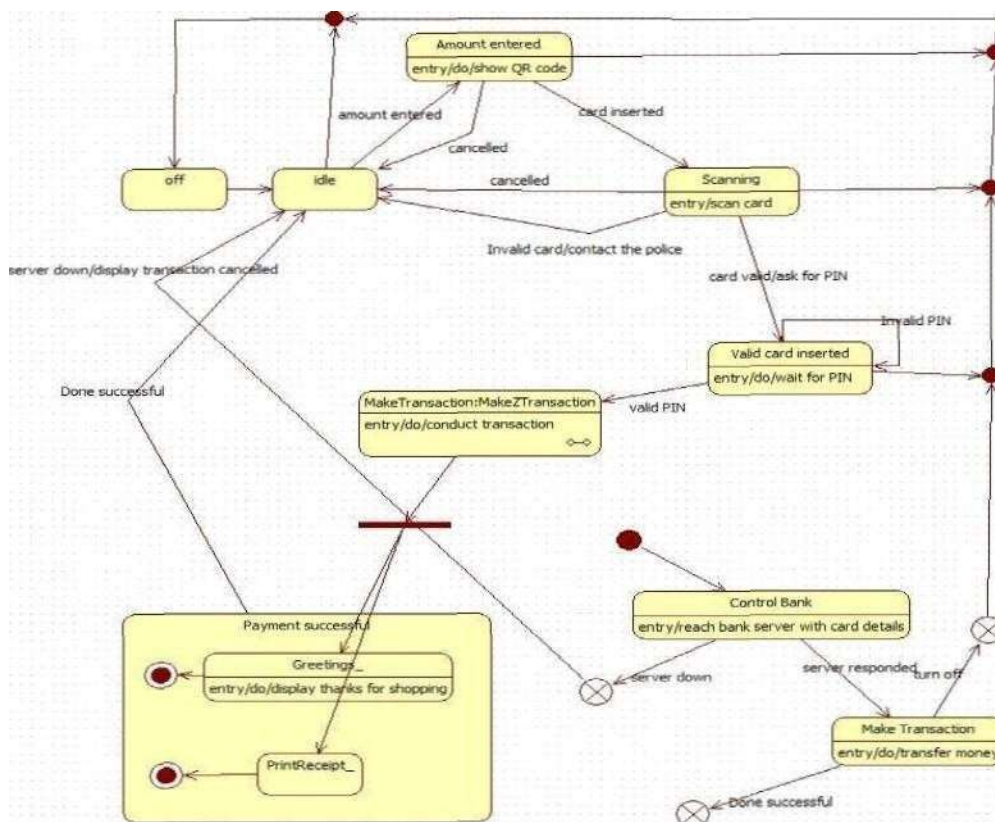
Fig 2.3 Advanced state diagram CCMS
