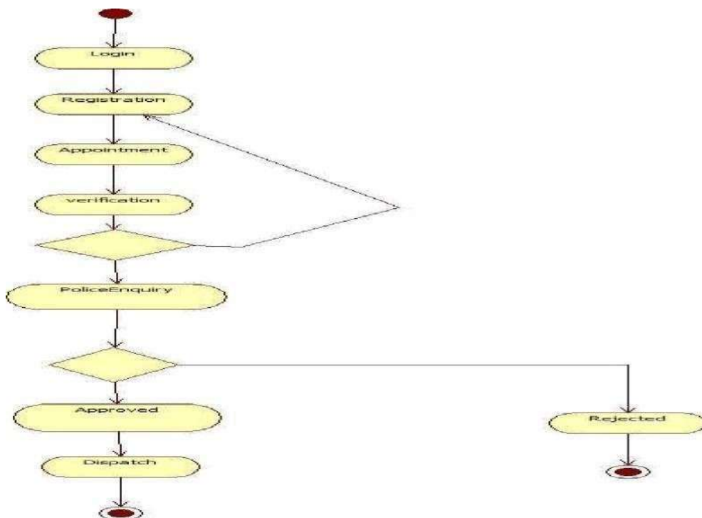
Fig 5.9 Advanced activity diagram PAS
