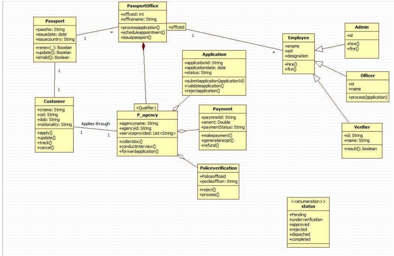
Fig 5.1 Class Diagram for Passport Automation System
