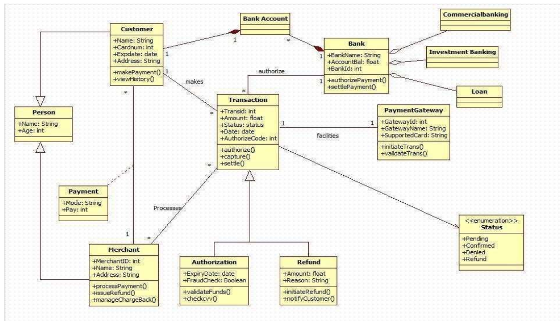
Fig 2.1 Class Diagram for Credit card management system
