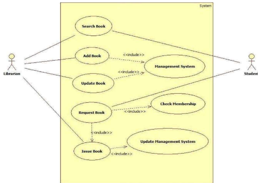
Fig 3.4 Simple Use Case Diagram LMS
