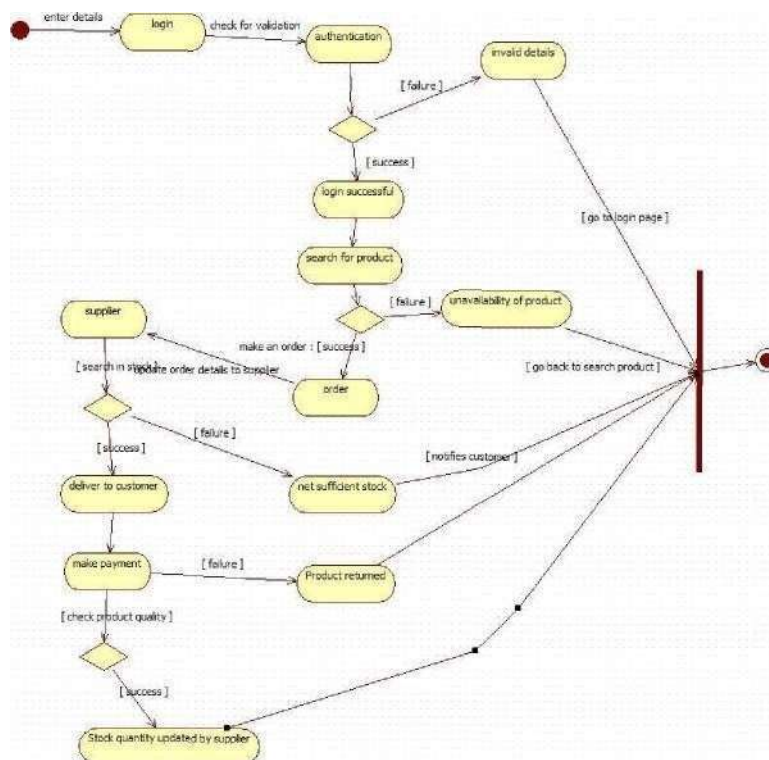
Fig 3.8 Simple Activity diagram SMS
