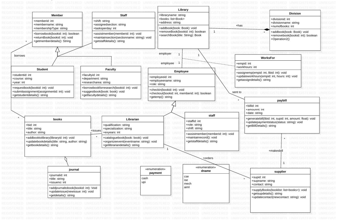
Fig 3.1 Class Diagram Library management System
