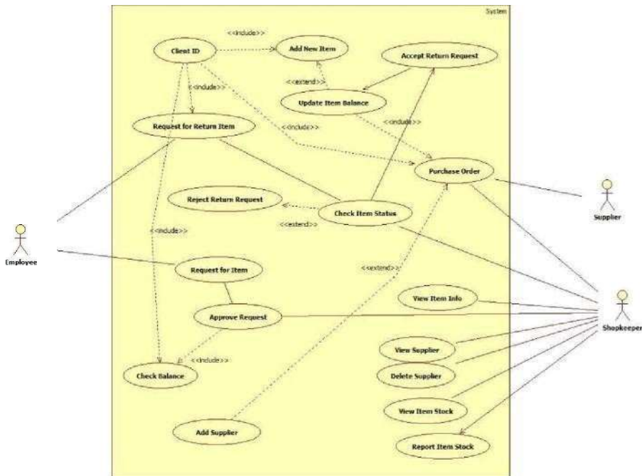
Fig 3.5 Advanced Use Case Diagram SMS
