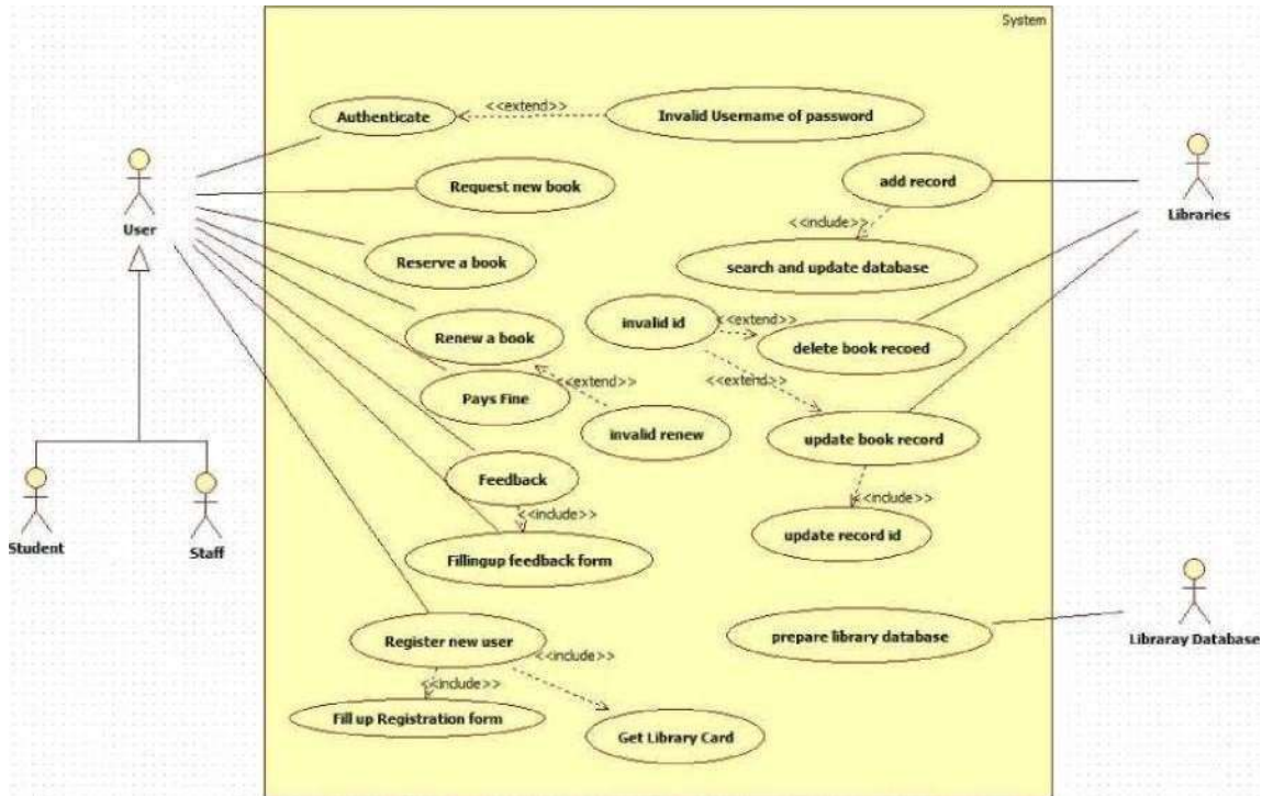
Fig 3.5 Advanced Use Case Diagram LMS
