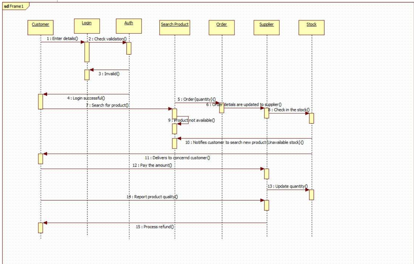
Fig 3.7 Sequence Diagram SMS
