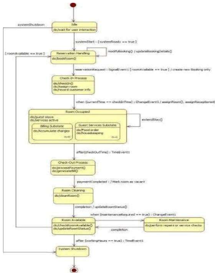
Fig 1.2 Simple State Diagram Hotel Management System
