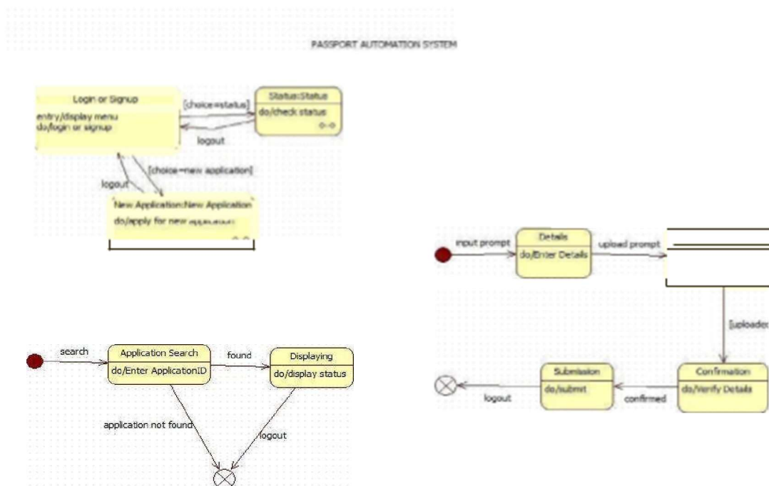
Fig 5.3 Advanced state diagram PAS
