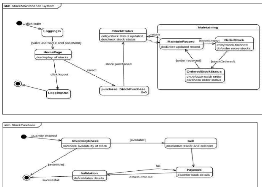
Fig 3.3 Advanced State Diagram SMS
