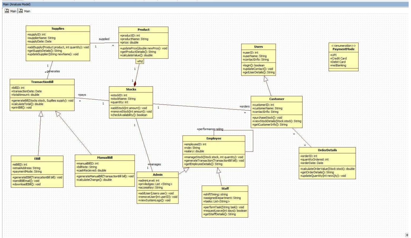
Fig 4.1 Class Diagram Stock Management System
