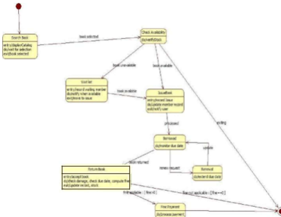
Fig 3.2 Simple state diagram LMS
