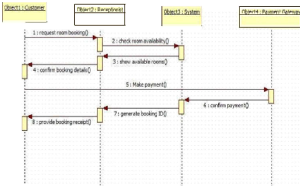
Fig 1.6 Simple Sequence Diagram for HMS
