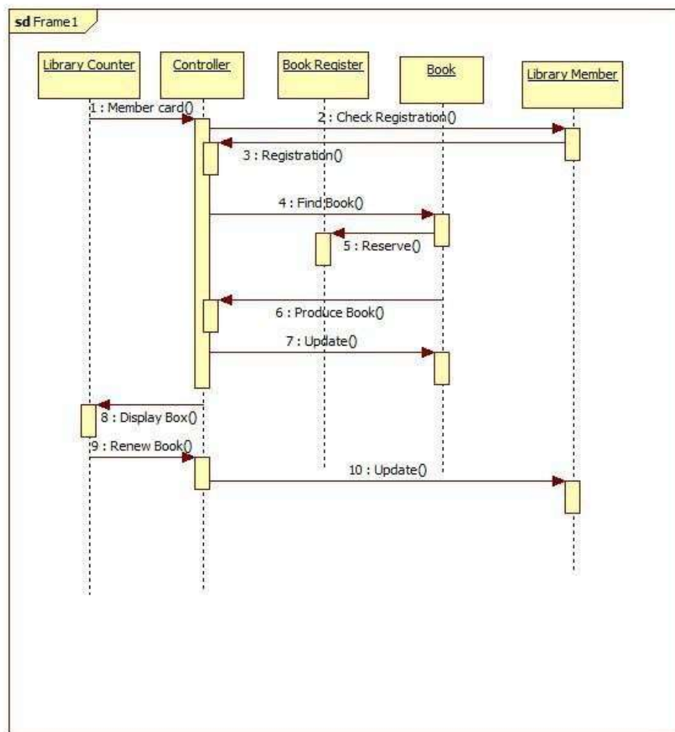
Fig 3.7 Advanced sequence diagram LMS
