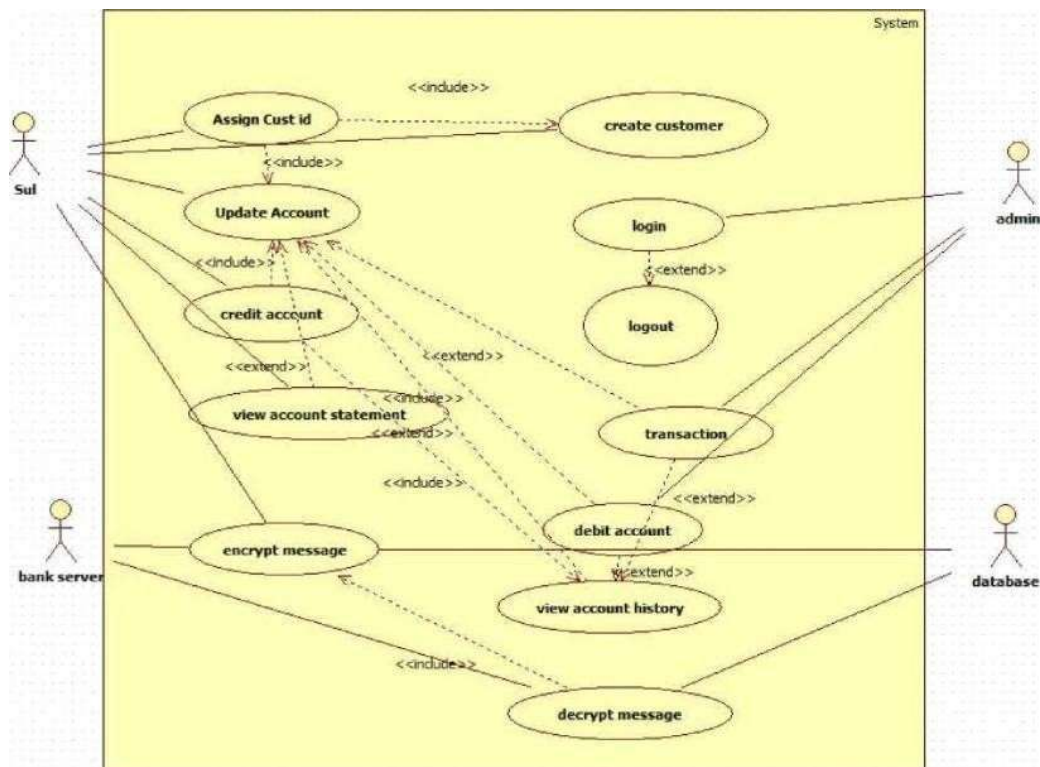
Fig 2.5 Advanced Use case Diagram CCMS
