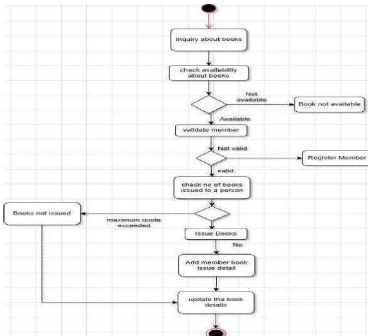
Fig 3.9 Advanced Activity Diagram LMS
