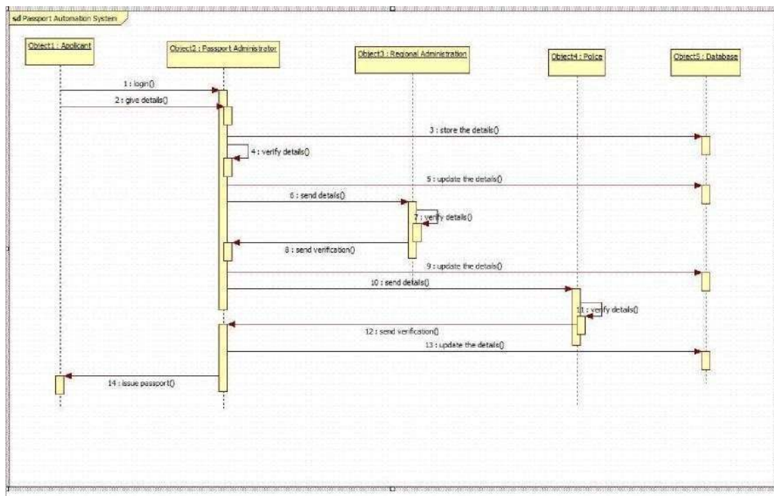
Fig 5.7 Advanced sequence diagram PAS
