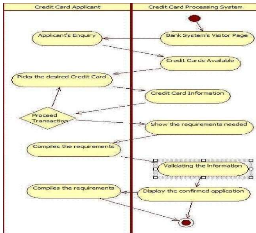
Fig 2.8 Simple Activity Diagram CCMS
