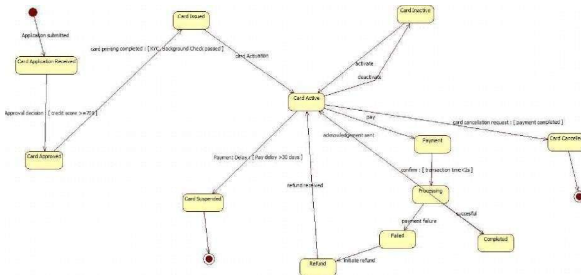
Fig 2.2 Simple state diagram CCMS
