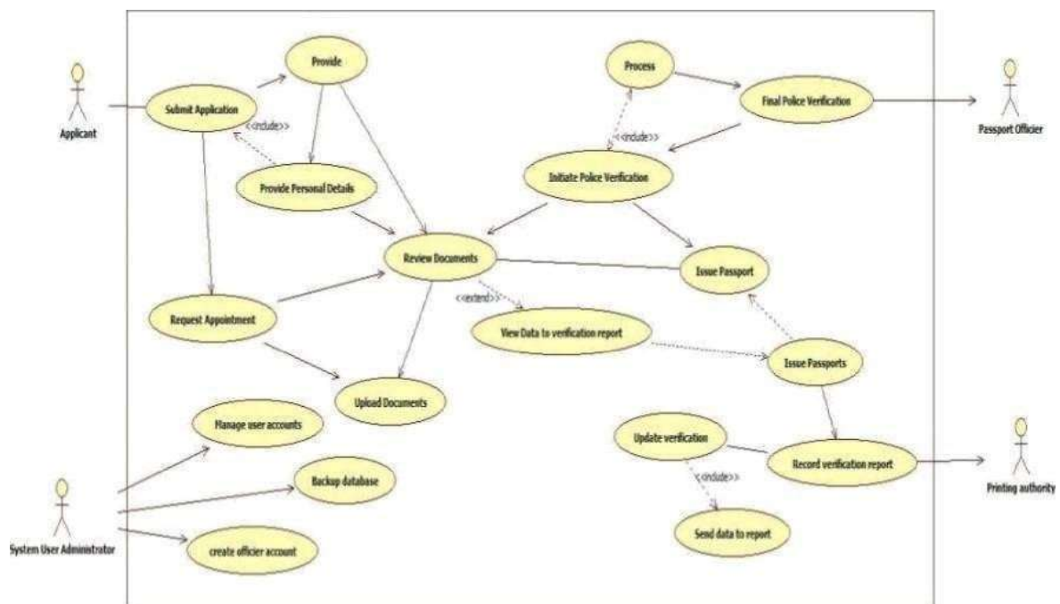
Fig 5.5 Advanced Use case diagram PAS
