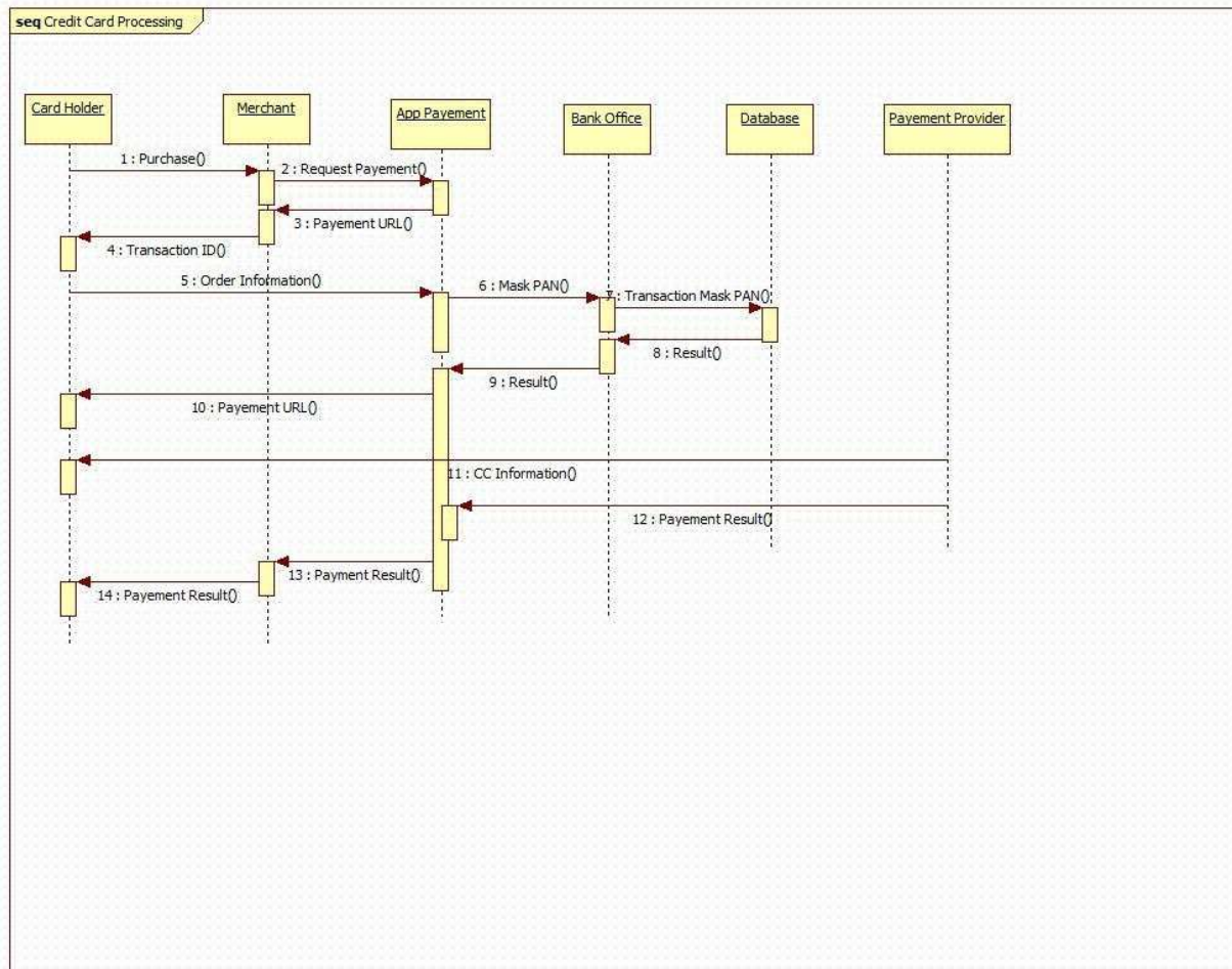
Fig 2.6 sequence diagram CCMS
