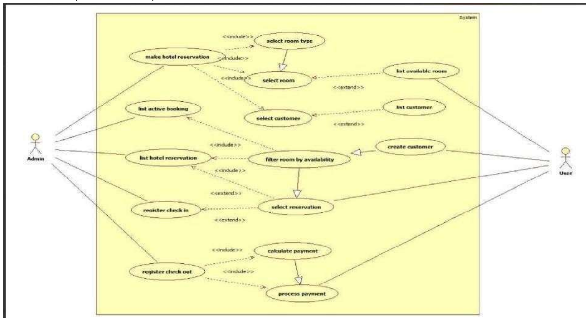
Fig 1.5 Advanced use case Diagram for HMS
