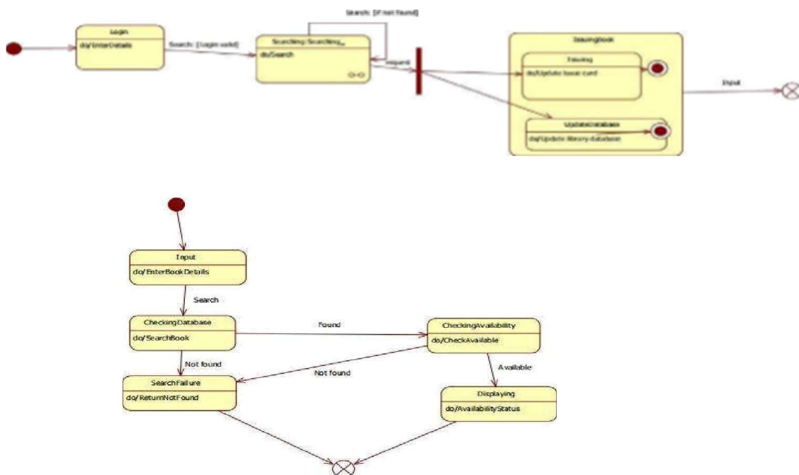
Fig 3.3 Advanced state diagram LMS
