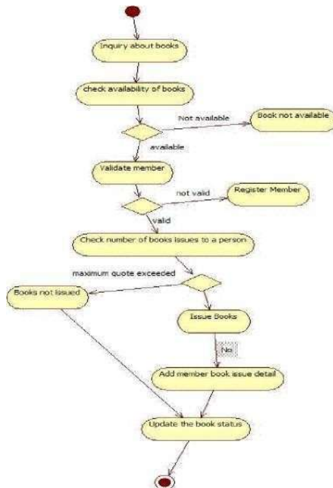
Fig 3.8 Simple Activity Diagram LMS
