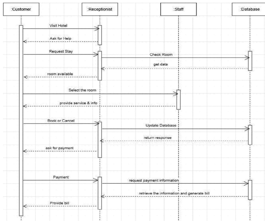
Fig 1.7 Advanced Sequence diagram HMS
