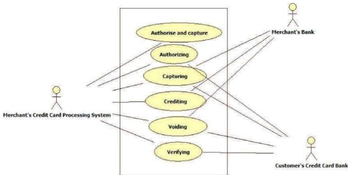
Fig 2.4 Simple Use case diagram for CCMS
