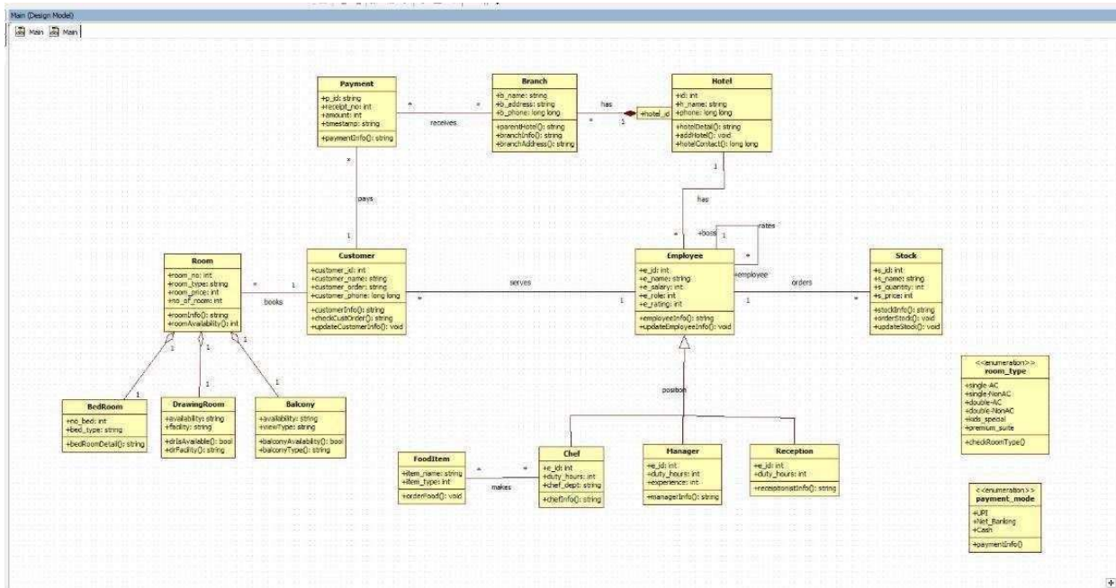
Fig 1.1 Class Diagram Hotel Management System
